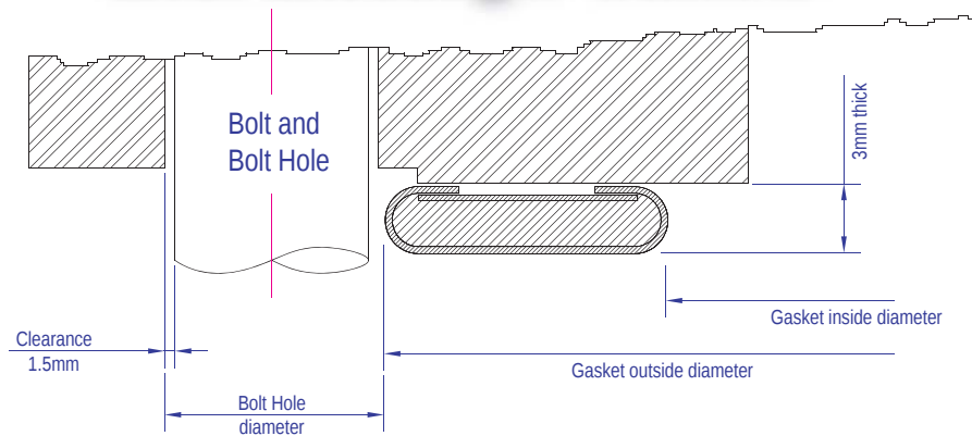
DIMENSIONS FOR JACKETED GASKETS USED WITH ASME/ANSI B16.5 FLANGES
