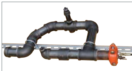
Burst pressure testing of DI threaded fittings (2')
