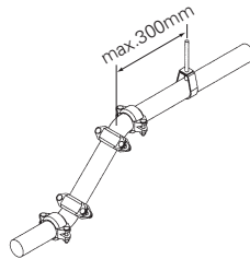
Short riser (or short drop)
