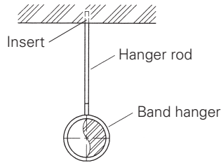
A rod hanger for a single pipe run
