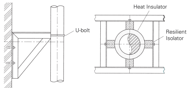
Sway brace ( ⊕ )
